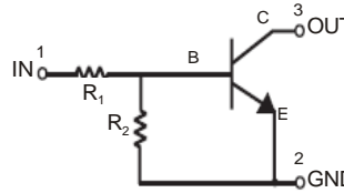
Schematic and Pin Configuration
