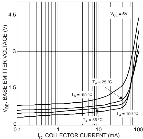
Fig. 4 Typical Base Emitter Voltage vs. Collector Current
