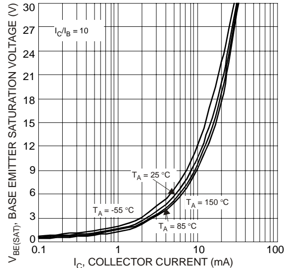
Fig. 17 Typical Base Emitter Saturation Voltage vs. Collector Current
