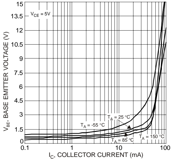
Fig. 16 Typical Base Emitter Voltage vs. Collector Current
