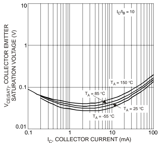
Fig. 7 Typical Collector Saturation Voltage vs. Collector Current
