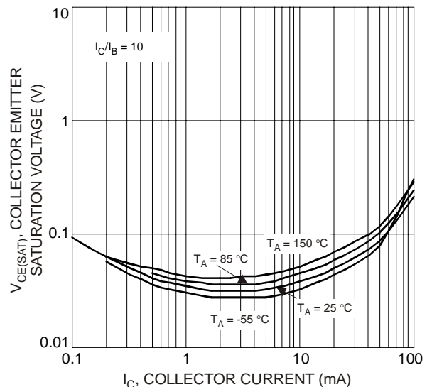
Fig. 19 Typical Collector Emitter Saturation Voltage vs. Collector Current
