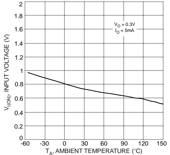
Fig. 3 Typical Input Voltage vs. Ambient Temperature
