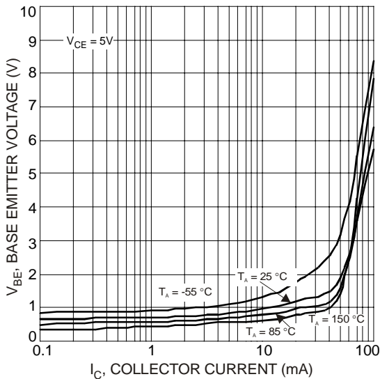
Fig. 10 Typical Base Emitter Voltage vs. Collector Current
