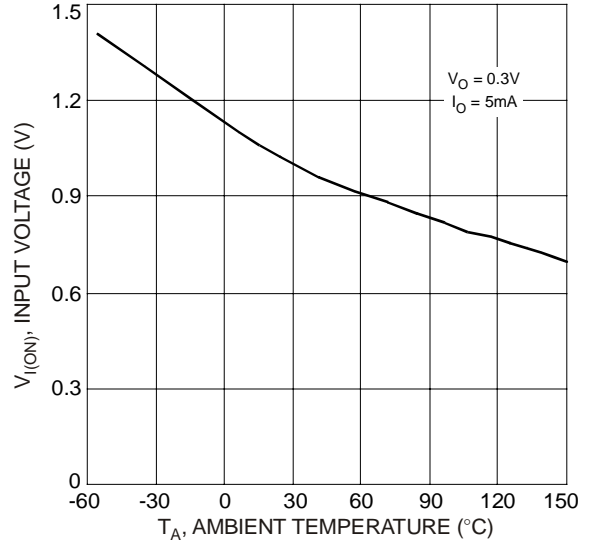
Fig. 15 Typical Input Voltage vs. Ambient Temperature
