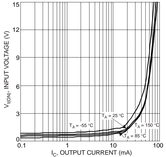
Fig. 9 Typical Input Voltage vs. Output Current
