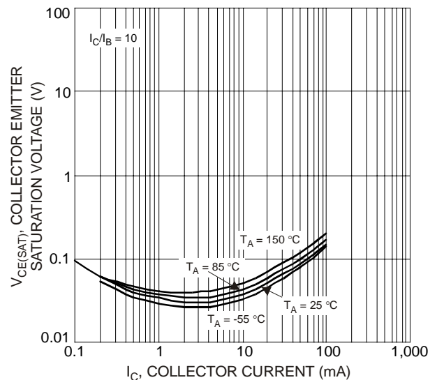
Fig. 13 Typical Collector Emitter Saturation Voltage vs. Collector Current
