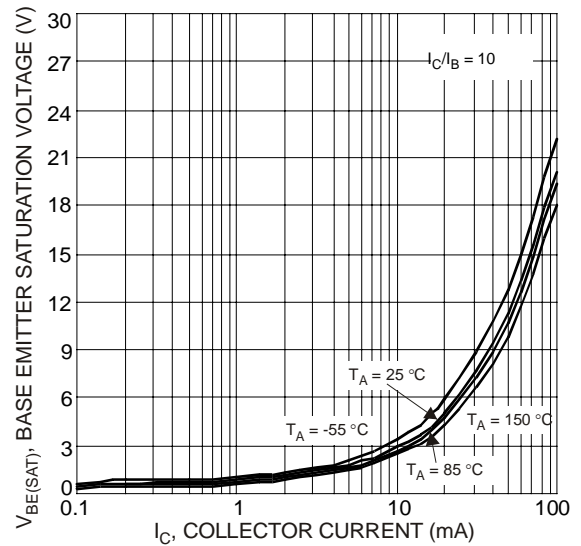
Fig. 5 Typical Base Emitter Saturation Voltage vs. Collector Current
