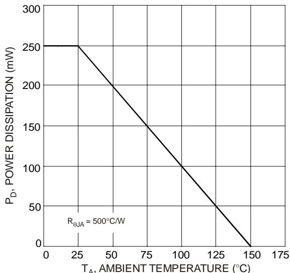
Fig. 1 Power Derating Curve (Note 3)
