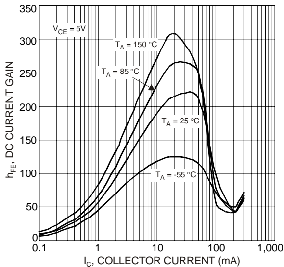
Fig. 18 Typical DC Current Gain vs. Collector Current
