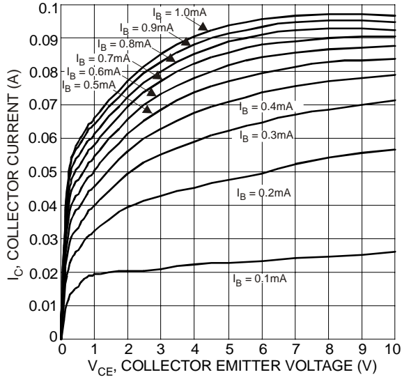
Fig. 14 Typical Collector Current vs. Collector Emitter Voltage
