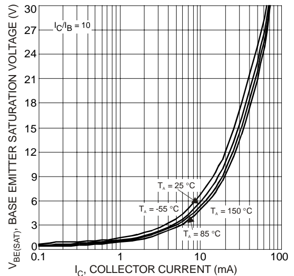
Fig. 11 Typical Base Emitter Saturation Voltage vs. Collector Current
